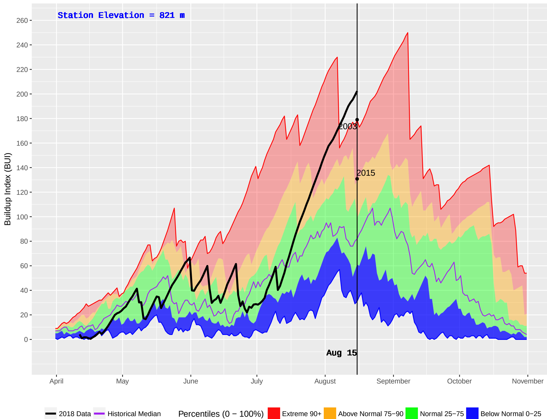
AKOKLI CREEK (838) : Historical (2003–2016) and Current (2018) Daily Buildup Index (BUI)
