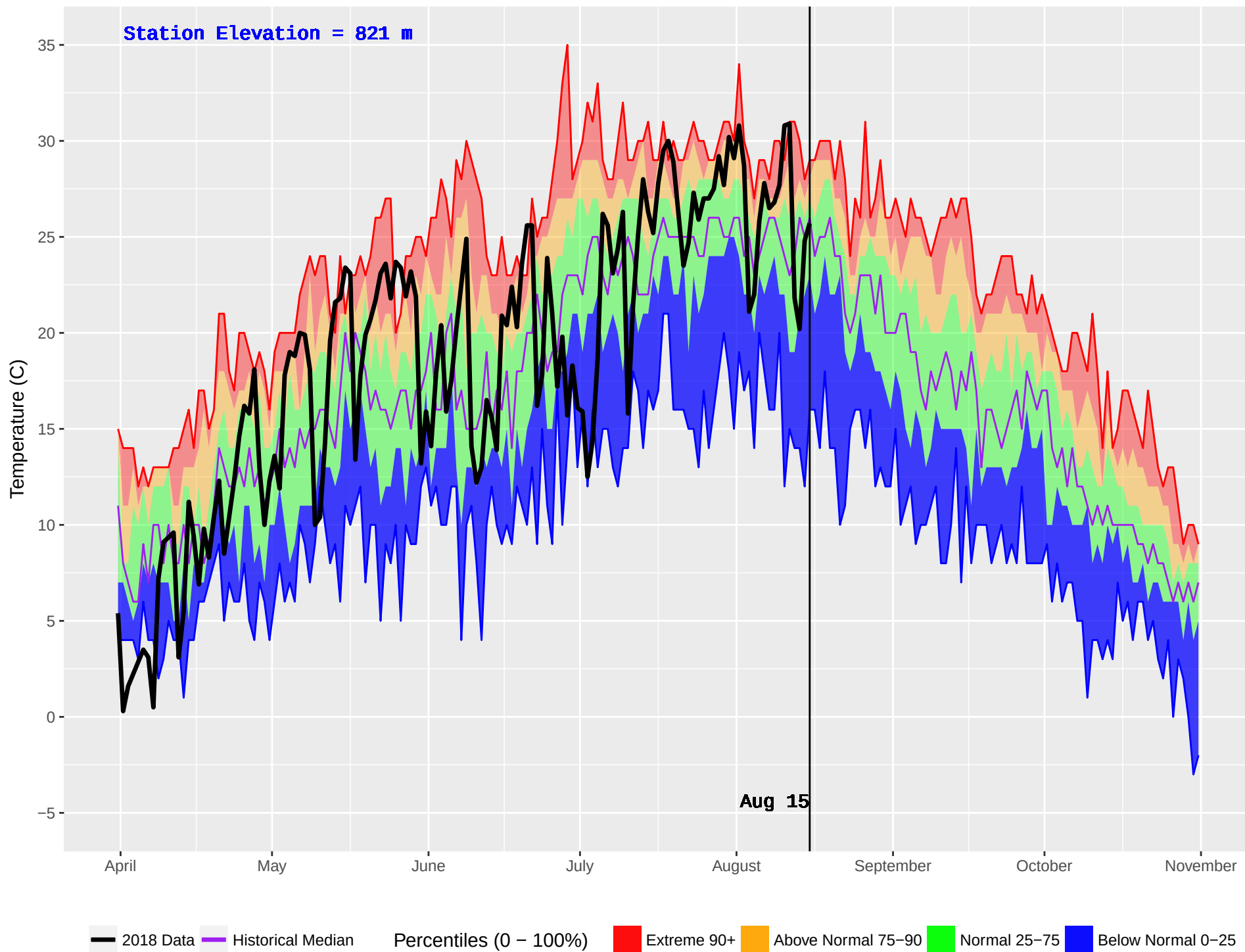
AKOKLI CREEK (838) : Historical (2003–2016) and Current (2018) Daily Temperature
