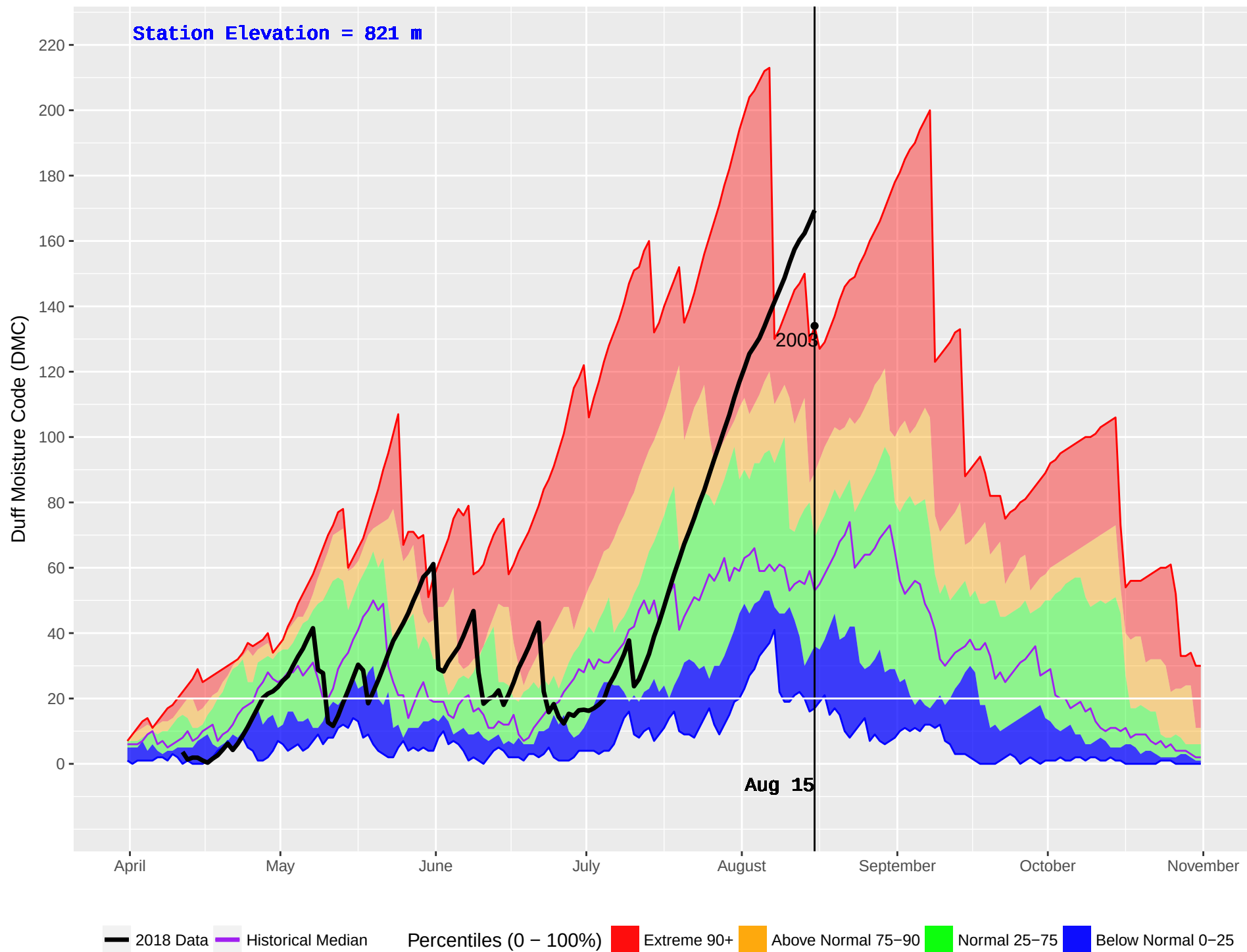
AKOKLI CREEK (838) : Historical (2003–2016) and Current (2018) Daily Duff Moisture Code (DMC)
